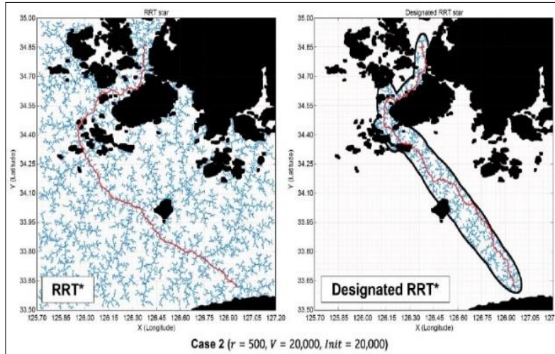
Fig. 2 Route planning
